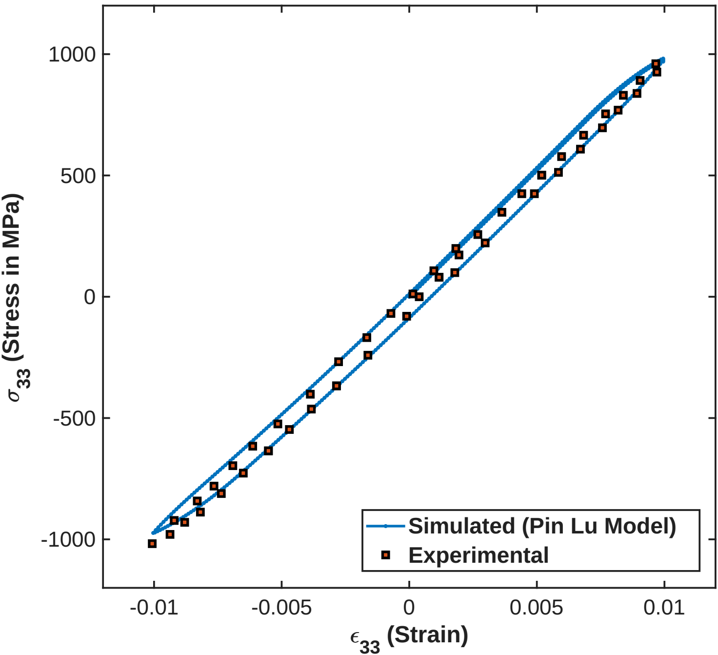
Cyclic Test upto 1% strain
